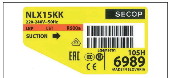
Fig.1 RoHS symbol on fixed speed compressor (type label)
