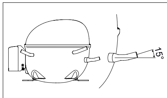
Fig. 2 Suction connector with 15° angle
