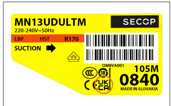
Fig.2 UKCA marking on a Secop compressor type label
