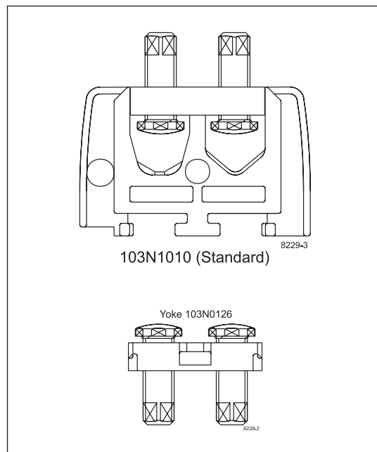
Fig. Cable fixture (cord relief) for P/T/D/N/F/S-Series compressors
