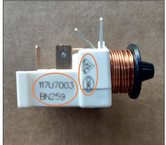
Fig.1 117U7xxx starting relay manufactured by Secop s.r.o (Slovakia)
