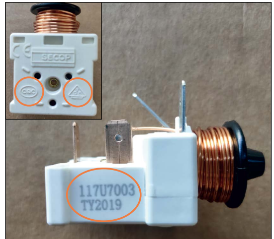
Fig.2 117U7xxx starting relay manufactured by Changshu Tianyin Electromechanical Co., Ltd.
