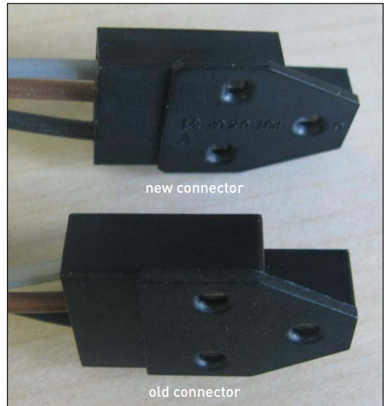
Fig.1 New connector and old connector for 117 CSR electrical equipment
