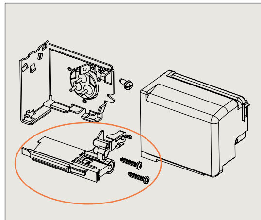
Fig. 1 K-Series' cable clamp mounting position
