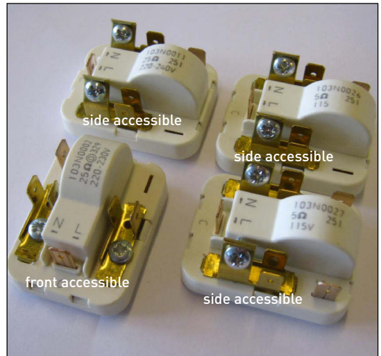
Fig.1 PTC starting devices with front and side accessible screw connections
