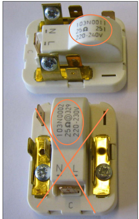
Fig.2 Example: PTC starting device 103N0002 to be replaced by PTC starting device 103N0011
