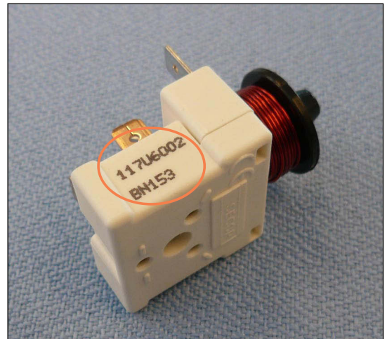
Fig.2 117U6xxx starting relay manufactured in Slovakia
