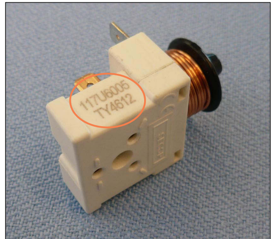
Fig.1 117U6xxx starting relay manufactured in China
